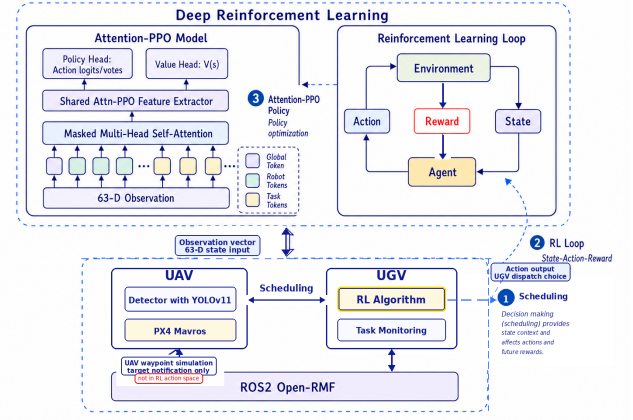
Fig. 2. UAV-assisted UGV dispatching architecture in the Open-RMF airport-terminal simulation. The RL policy dispatches UGVs; UAV simulation supports target discovery and task notification.
