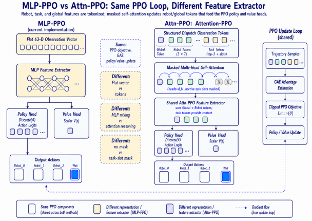
Fig. 1. MLP-PPO and Attn-PPO with different feature extractors.
